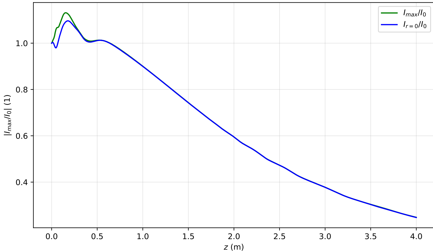
I_{max}(x = 0, y = 0, z)/I_0 , \text{Pin}=0.2\text{Pcr} , noisy input, artificial time
